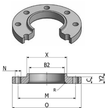
Flange Lap Joint
