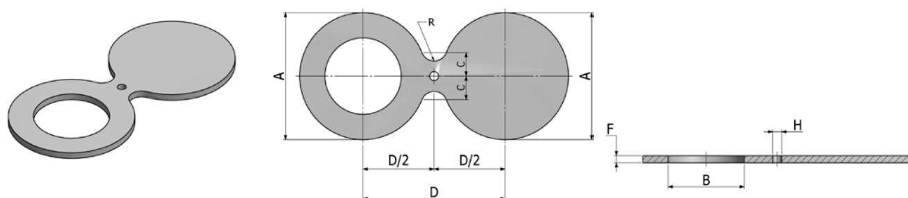
Figura 8 Face RF N120
