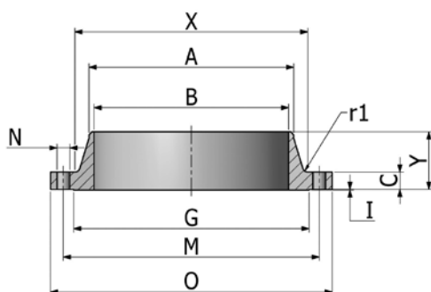
Flange FWN
