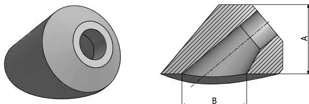
Colar BW
