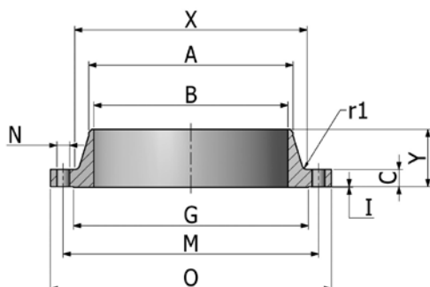
Flange FWN
