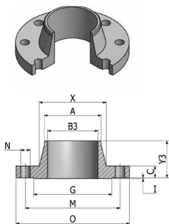
Flange FWN
