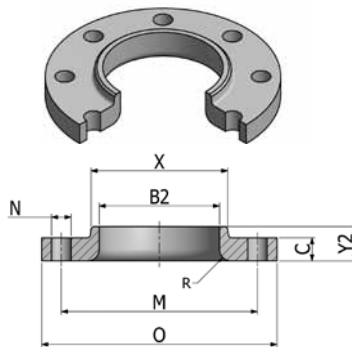
Flange Lap Joint
