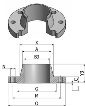
Flange FWN
