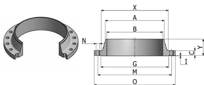
Flange FWN
