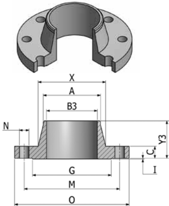
Flange FWN
