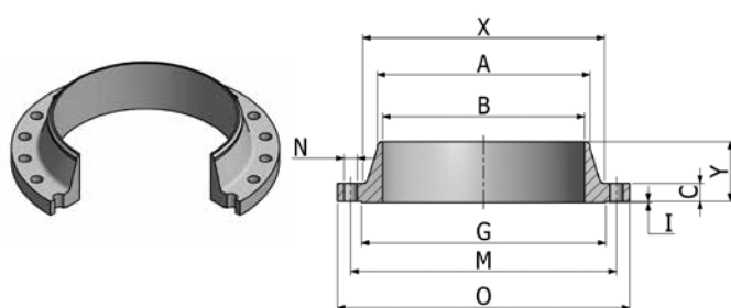
Flange FWN
