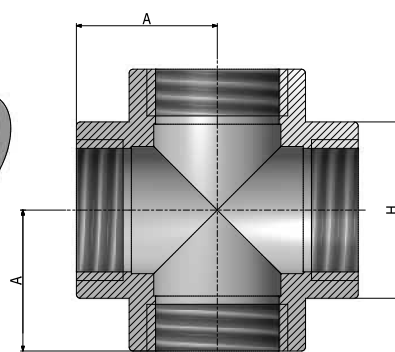
Cruzeta
