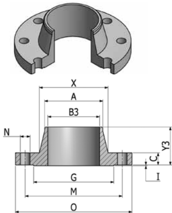
Flange FWN
