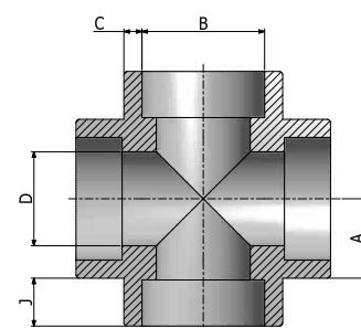
Cruzeta
