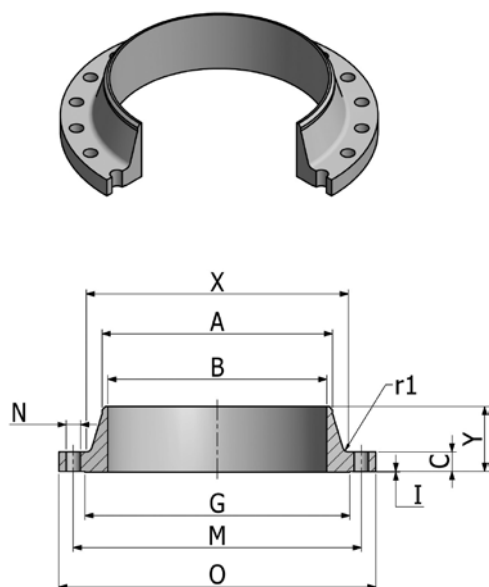
Flange FWN
